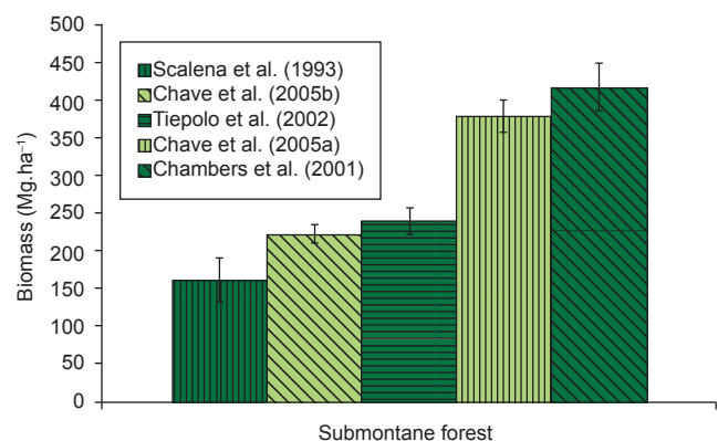
Figure 4. AGB for submontane Mata Atlântica plots. Error bars represent standard deviation. The biomass was estimated according models with one (DBH), two (DBH and height) or three (DBH, height and wood density) variables. The tree height was estimated using H = 1.9541 \times \text{DBH}^{0.5982} (Figure 3b)
